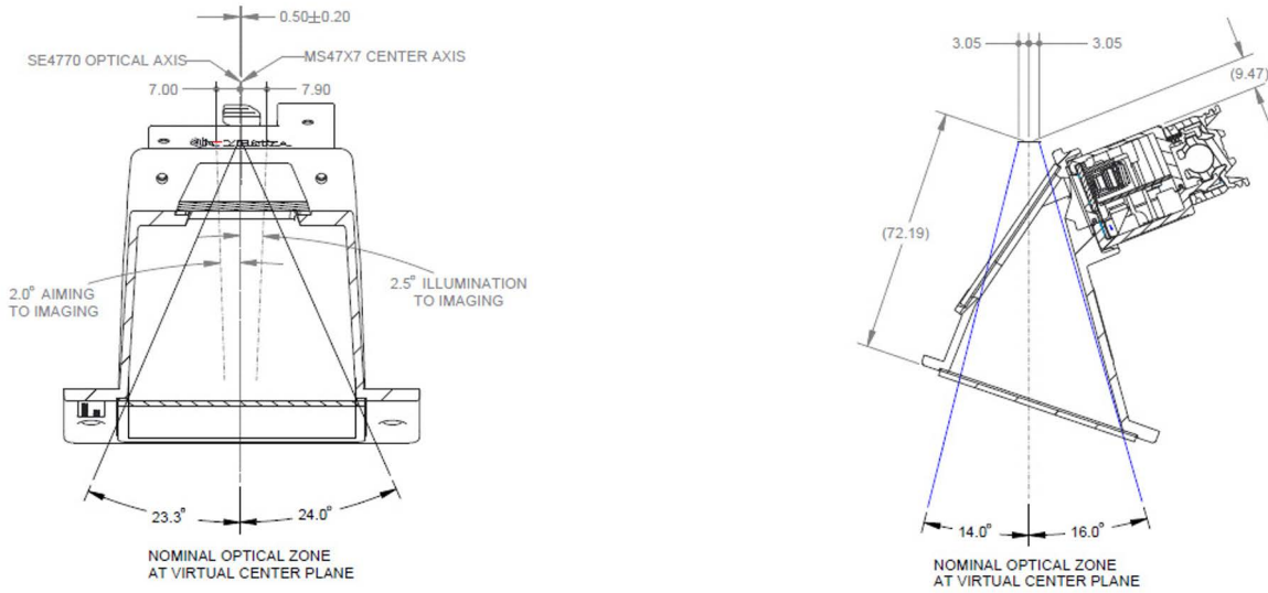
Figure 14 MS4777 Cone Imaging Optical Zone at Exit Window
