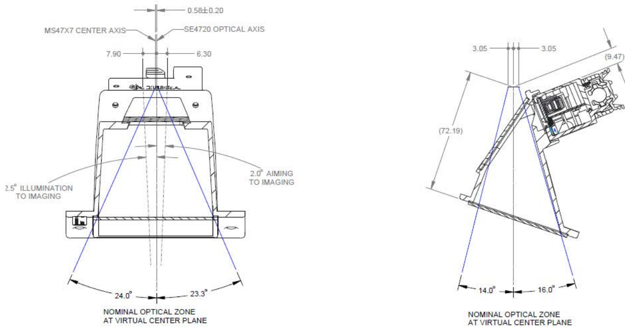
Figure 13 MS4727 Cone Imaging Optical Zone at Exit Window
