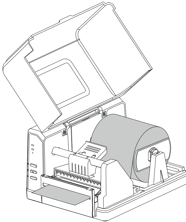
Figure 3-3 Cutter Mode
