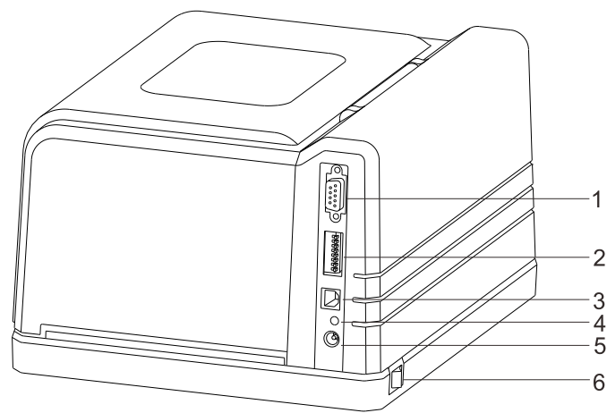
Figure 2-3 Rear View
